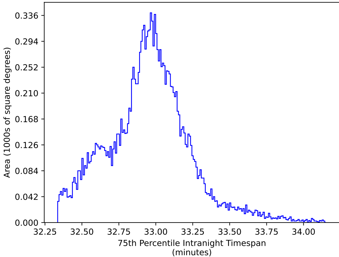
too_5_4v3.4_10yrs WFD y band: 75th Percentile Intranight Timespan
