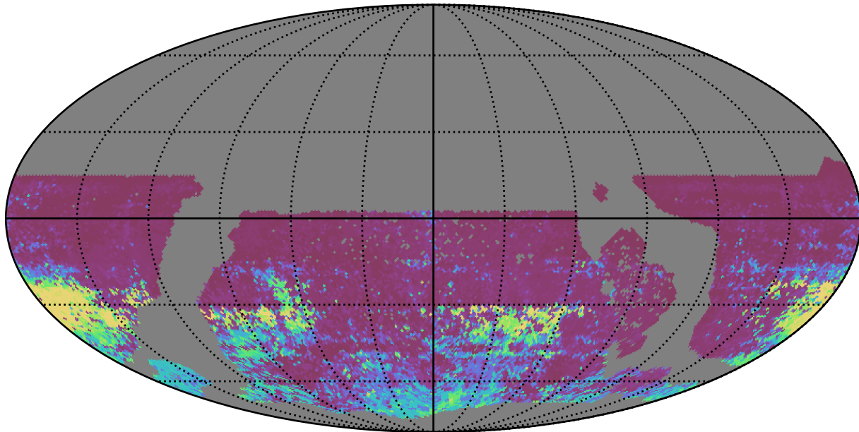
too_5_4v3.4_10yrs WFD r band: 75th Percentile Intranight Timespan
