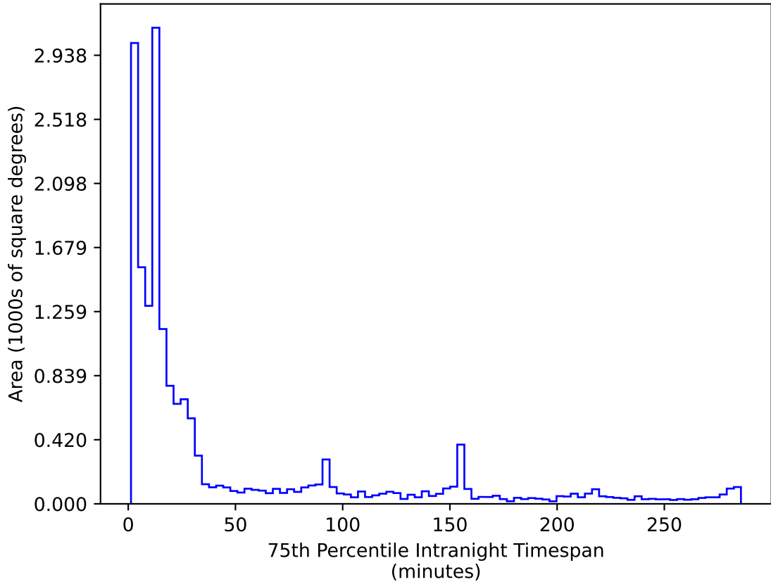
too_5_4v3.4_10yrs WFD r band: 75th Percentile Intranight Timespan
