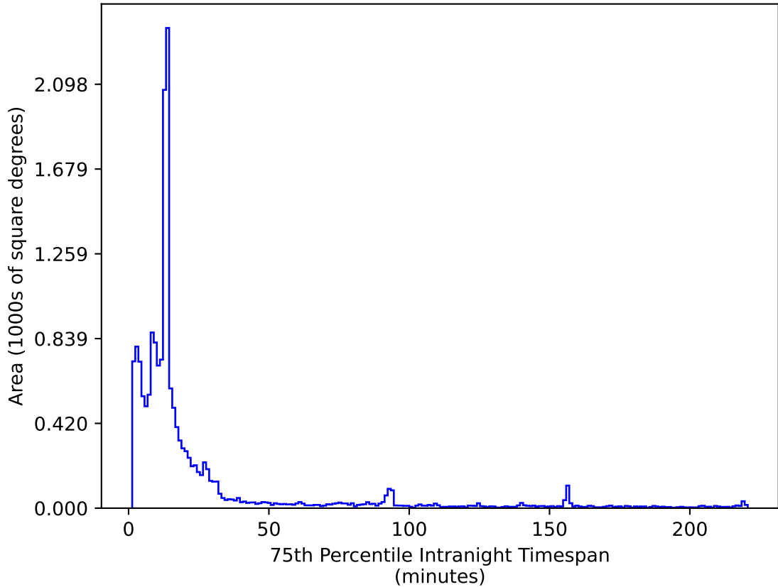
too_5_4v3.4_10yrs WFD i band: 75th Percentile Intranight Timespan
