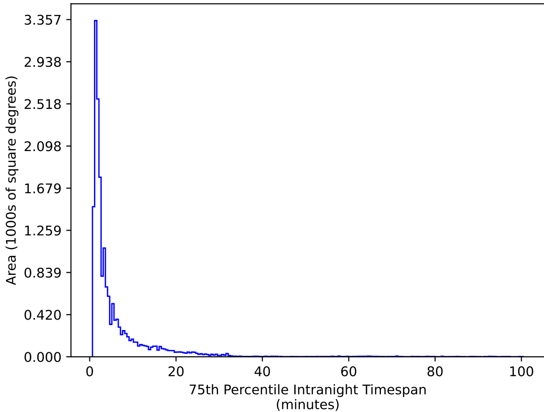
too_5_4v3.4_10yrs WFD g band: 75th Percentile Intranight Timespan
