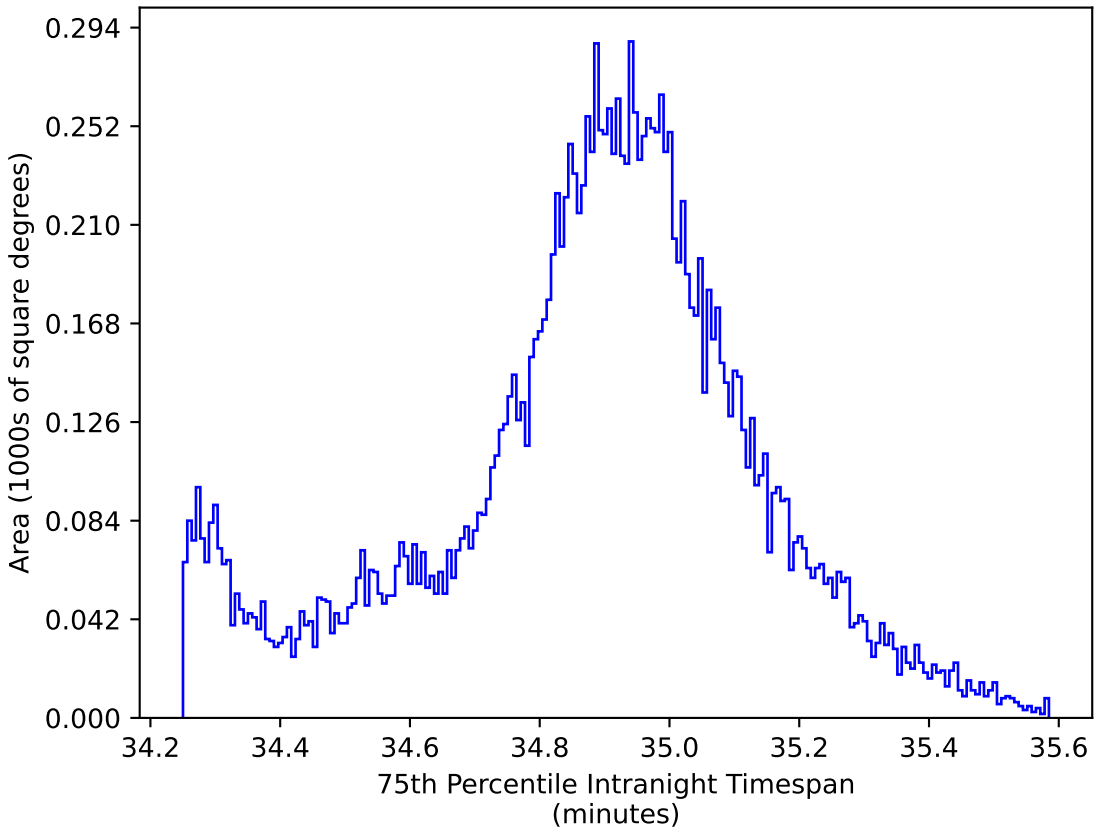
too_5_4v3.4_10yrs WFD all bands: 75th Percentile Intranight Timespan
