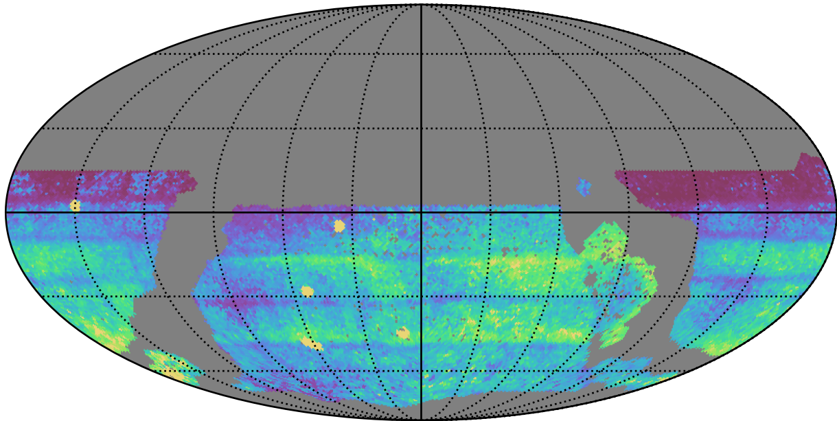
too_5_4v3.4_10yrs WFD: 75th Percentile Intranight Timespan
