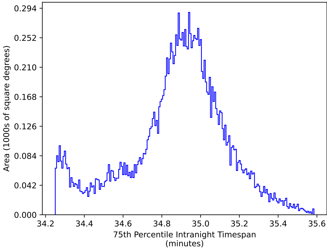
too_5_4v3.4_10yrs WFD: 75th Percentile Intranight Timespan
