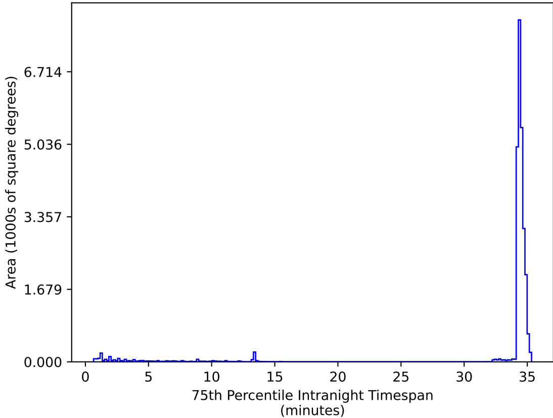
too_5_4v3.4_10yrs All sky zy bands: 75th Percentile Intranight Timespan
