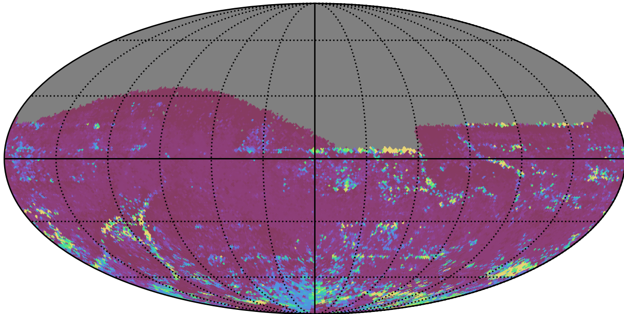
too_5_4v3.4_10yrs All sky z band: 75th Percentile Intranight Timespan
