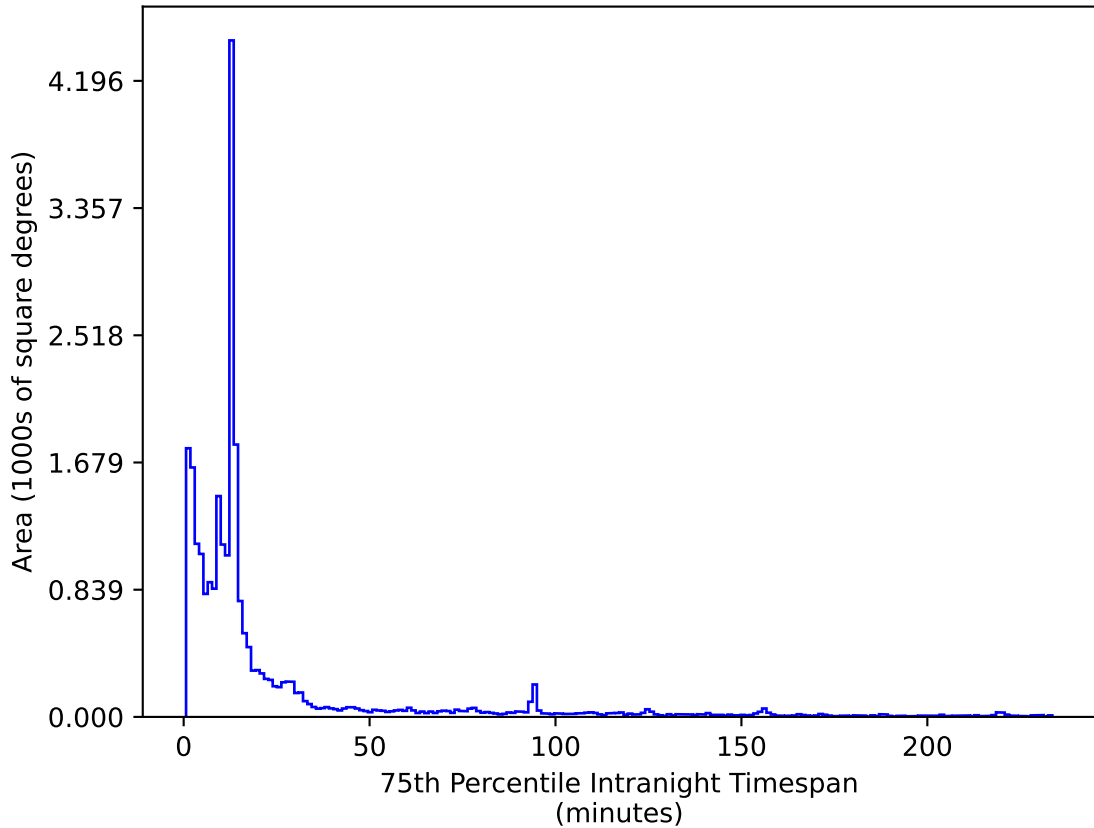
too_5_4v3.4_10yrs All sky z band: 75th Percentile Intranight Timespan
