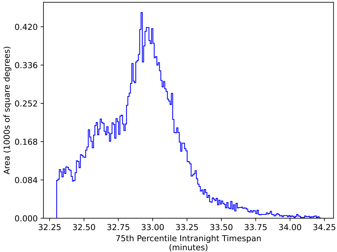
too_5_4v3.4_10yrs All sky y band: 75th Percentile Intranight Timespan
