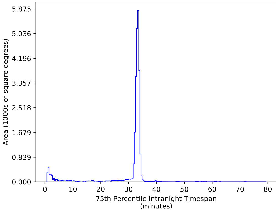
too_5_4v3.4_10yrs All sky ug bands: 75th Percentile Intranight Timespan
