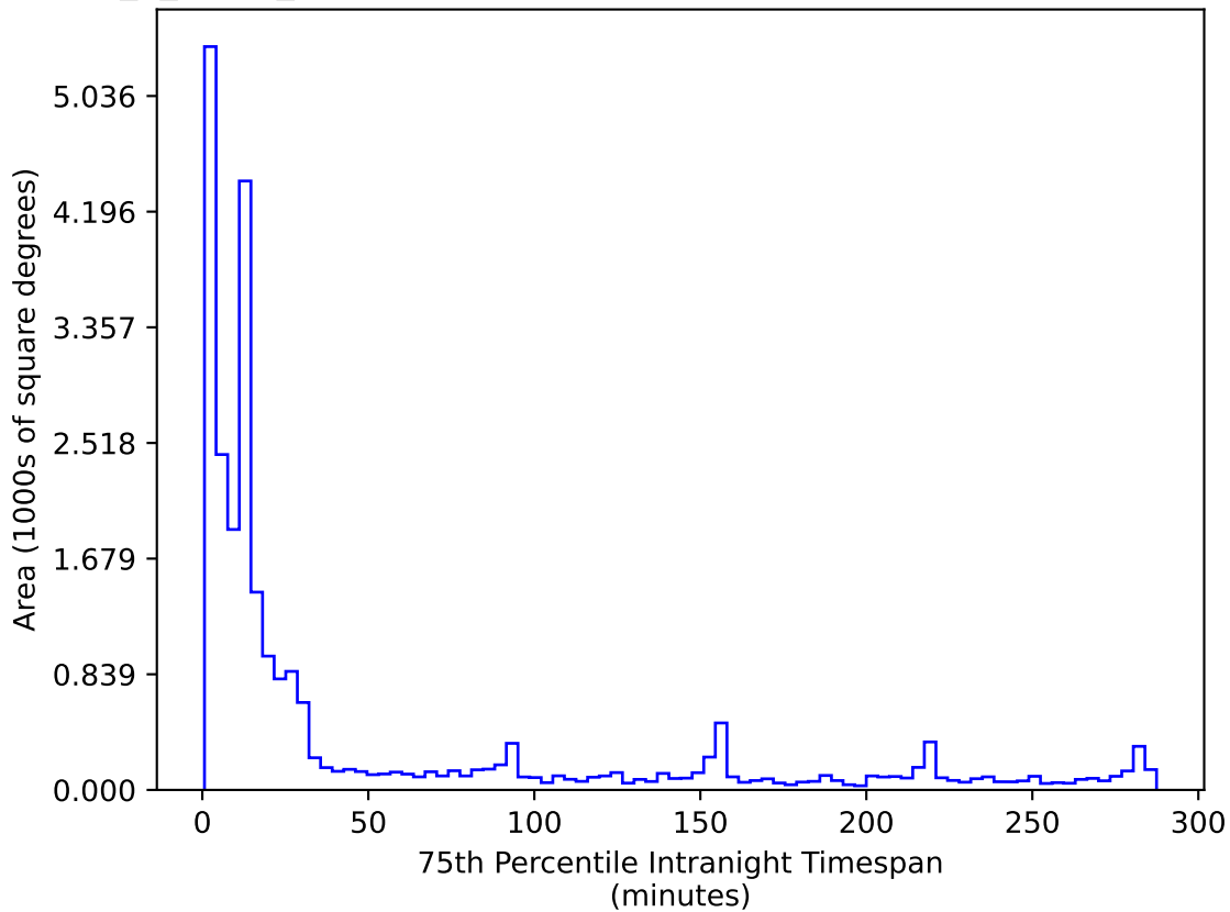
too_5_4v3.4_10yrs All sky r band: 75th Percentile Intranight Timespan
