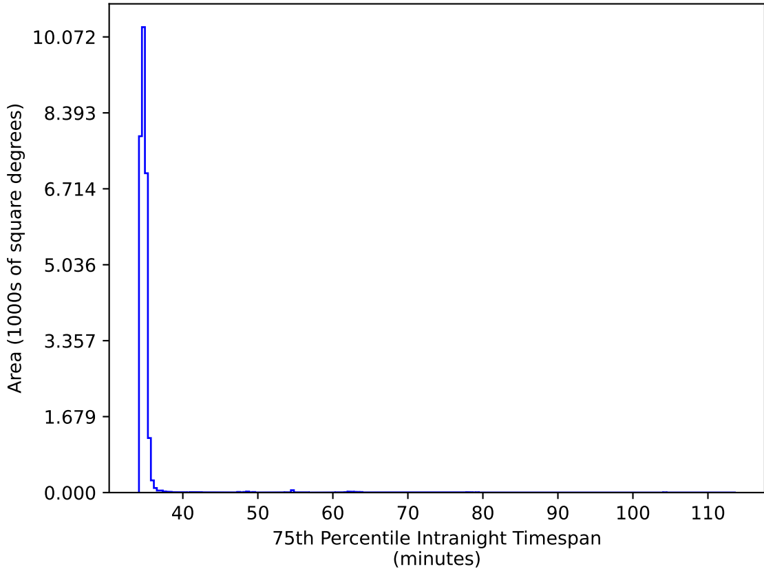
too_5_4v3.4_10yrs All sky iz bands: 75th Percentile Intranight Timespan
