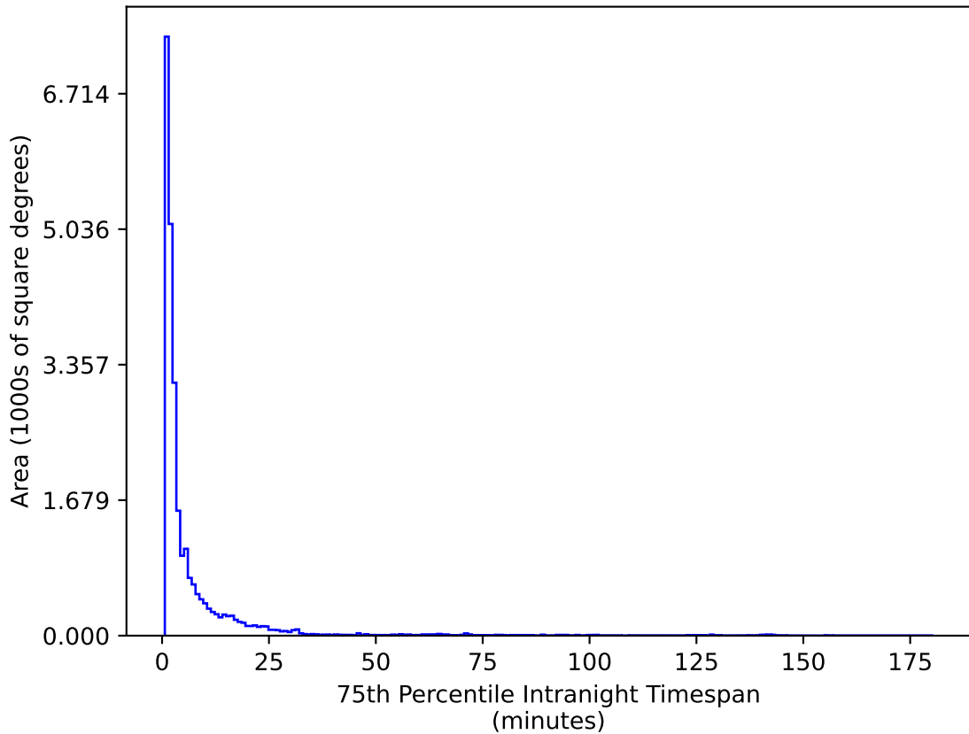
too_5_4v3.4_10yrs All sky g band: 75th Percentile Intranight Timespan
