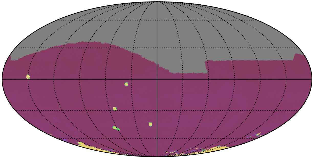
too_5_4v3.4_10yrs All sky: 75th Percentile Intranight Timespan
