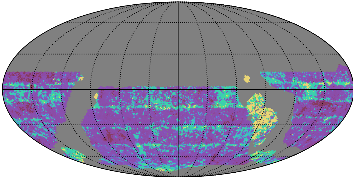
too_5_4v3.4_10yrs WFD z band: 20thPercentile Inter-Night Gap
