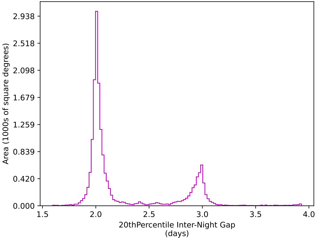
too_5_4v3.4_10yrs WFD z band: 20thPercentile Inter-Night Gap
