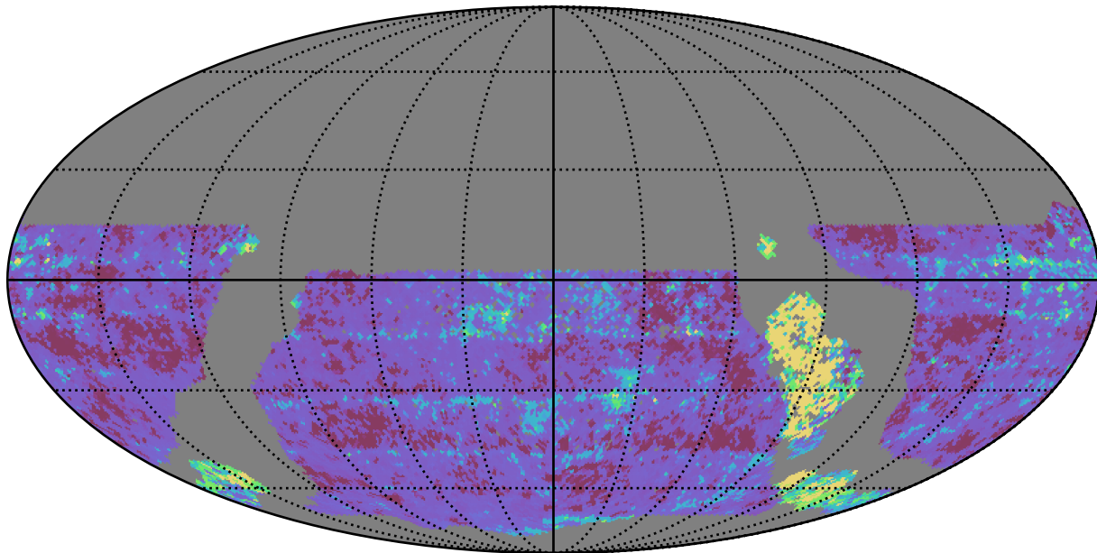
too_5_4v3.4_10yrs WFD y band: 20thPercentile Inter-Night Gap
