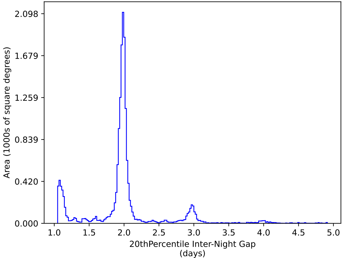
too_5_4v3.4_10yrs WFD y band: 20thPercentile Inter-Night Gap
