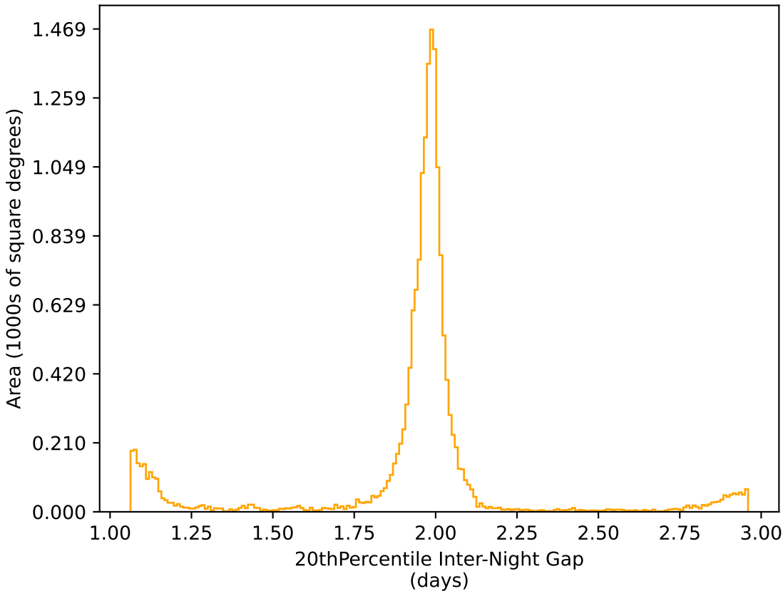
too_5_4v3.4_10yrs WFD r band: 20thPercentile Inter-Night Gap
