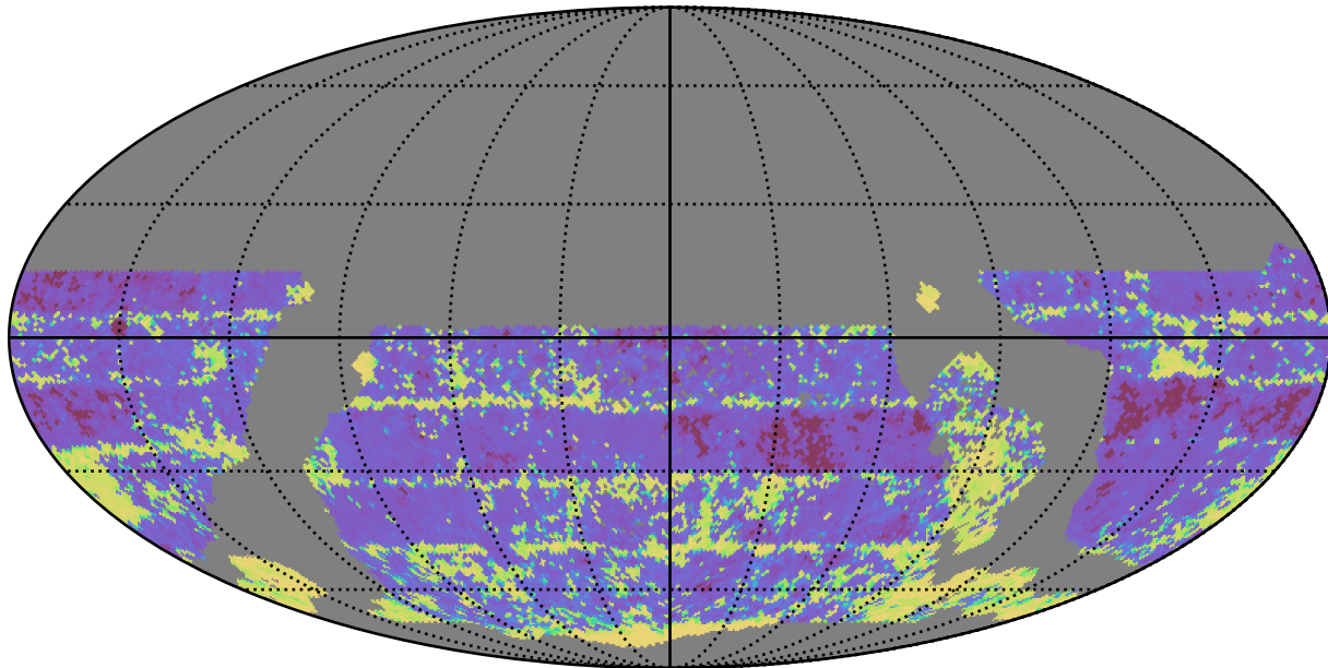
too_5_4v3.4_10yrs WFD i band: 20thPercentile Inter-Night Gap
