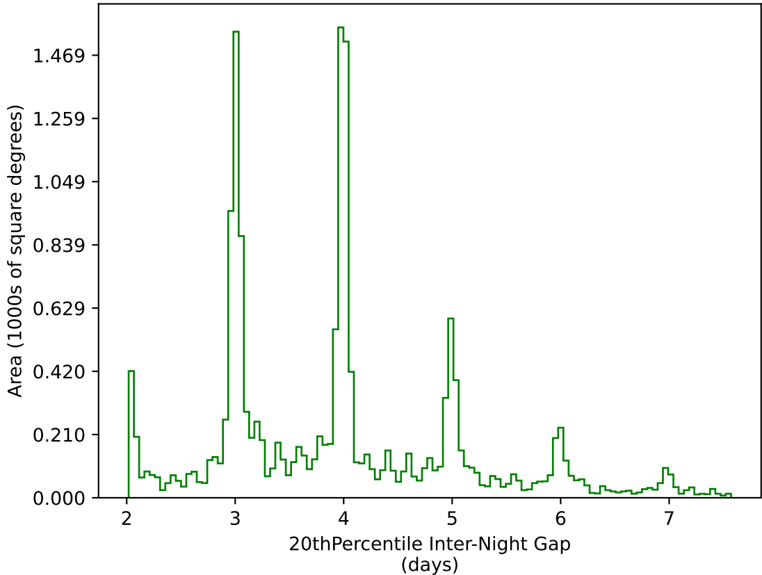
too_5_4v3.4_10yrs WFD g band: 20thPercentile Inter-Night Gap
