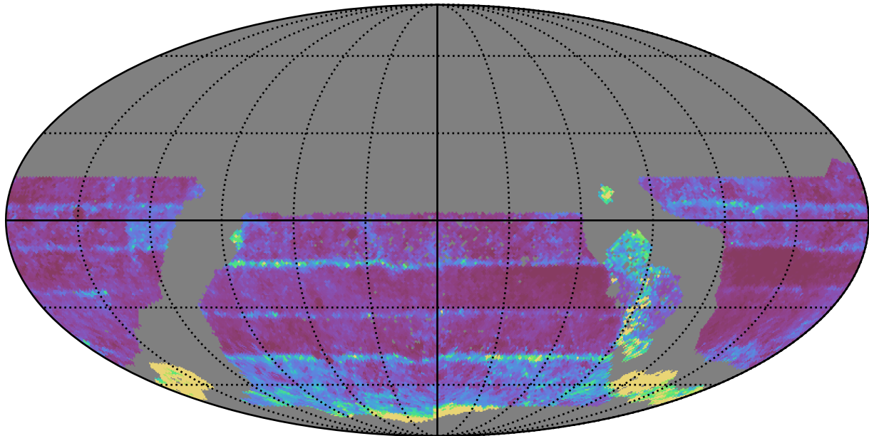
too_5_4v3.4_10yrs WFD all bands: 20thPercentile Inter-Night Gap
