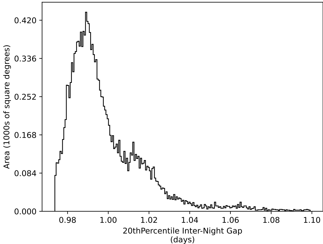
too_5_4v3.4_10yrs WFD all bands: 20thPercentile Inter-Night Gap
