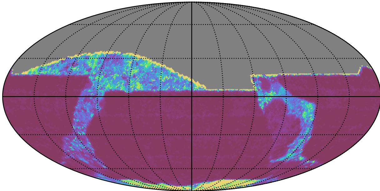
too_5_4v3.4_10yrs All sky z band: 20thPercentile Inter-Night Gap
