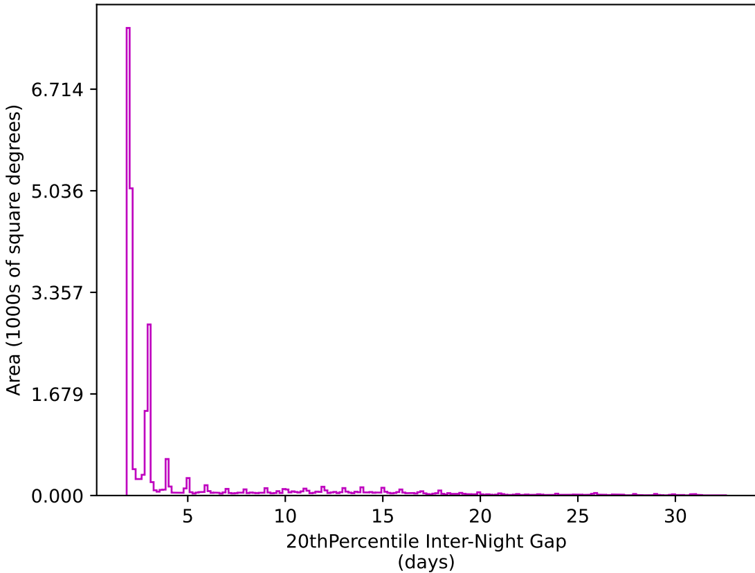
too_5_4v3.4_10yrs All sky z band: 20thPercentile Inter-Night Gap
