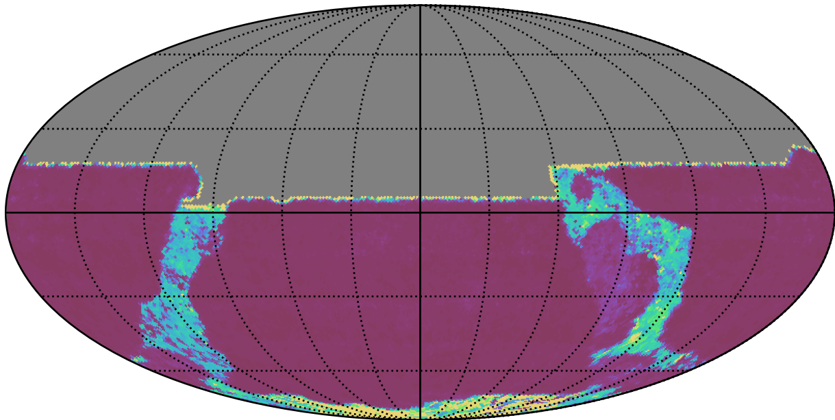
too_5_4v3.4_10yrs All sky y band: 20thPercentile Inter-Night Gap
