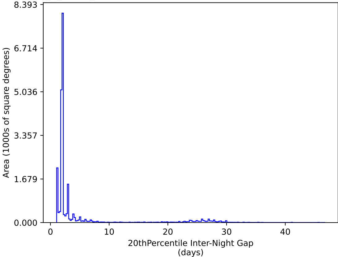
too_5_4v3.4_10yrs All sky y band: 20thPercentile Inter-Night Gap
