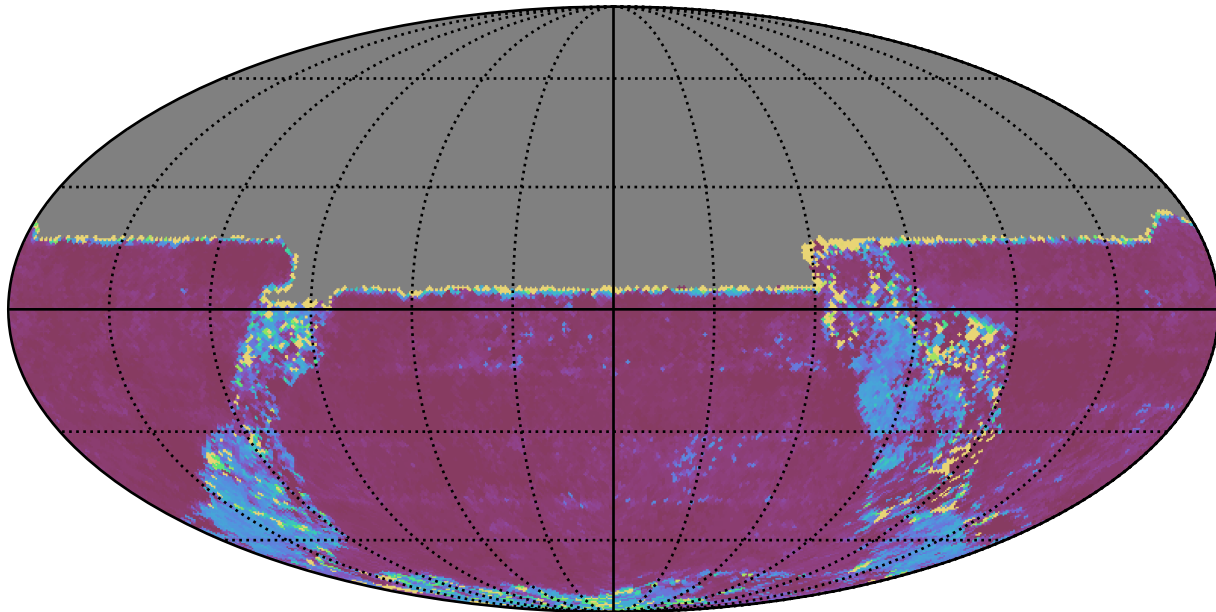
too_5_4v3.4_10yrs All sky u band: 20thPercentile Inter-Night Gap
