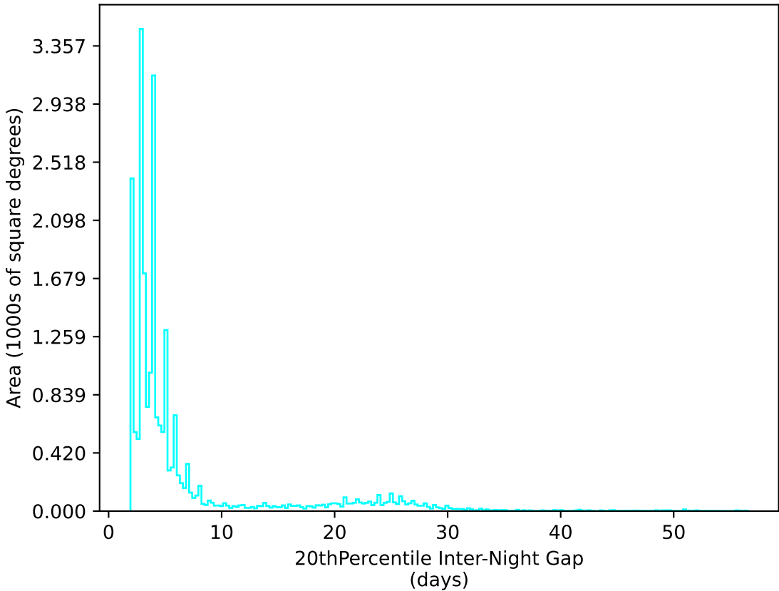
too_5_4v3.4_10yrs All sky u band: 20thPercentile Inter-Night Gap
