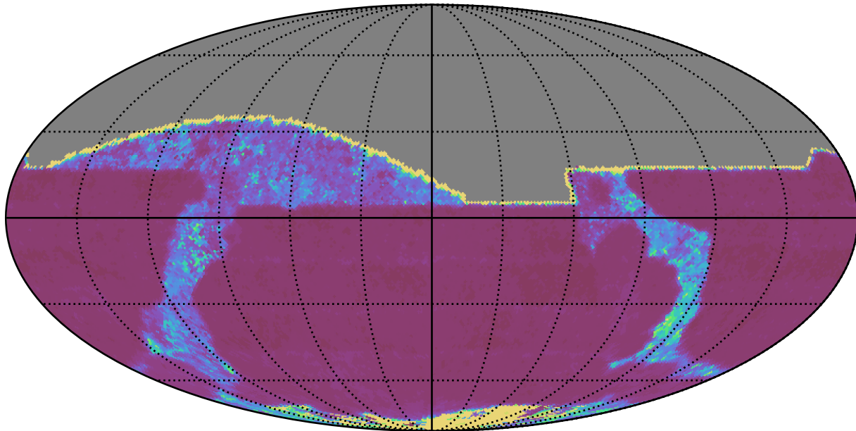
too_5_4v3.4_10yrs All sky r band: 20thPercentile Inter-Night Gap
