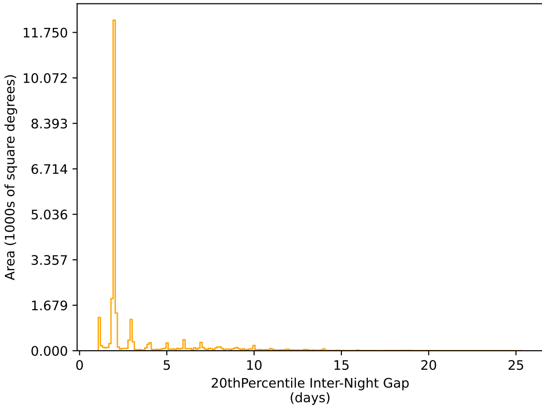
too_5_4v3.4_10yrs All sky r band: 20thPercentile Inter-Night Gap
