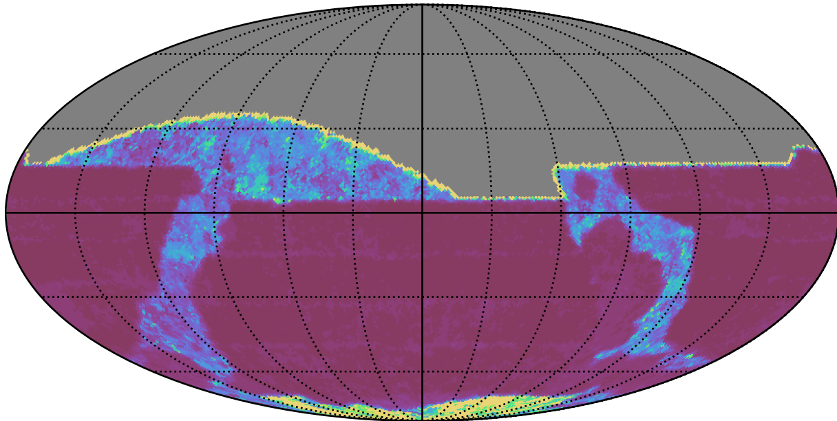
too_5_4v3.4_10yrs All sky i band: 20thPercentile Inter-Night Gap
