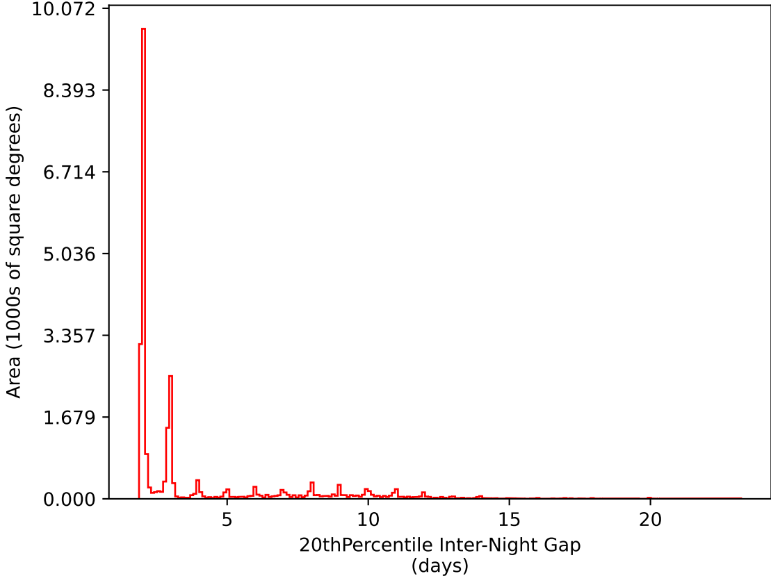
too_5_4v3.4_10yrs All sky i band: 20thPercentile Inter-Night Gap
