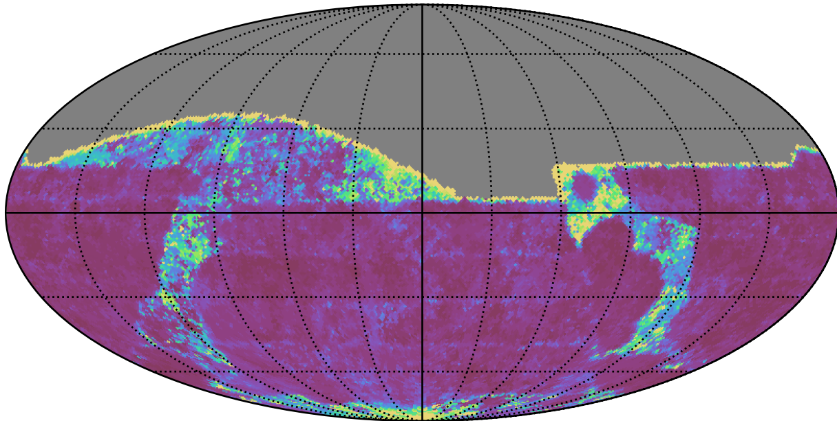
too_5_4v3.4_10yrs All sky g band: 20thPercentile Inter-Night Gap
