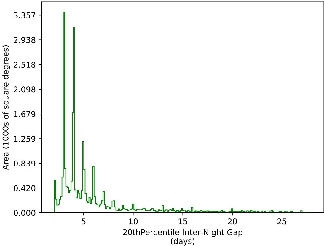
too_5_4v3.4_10yrs All sky g band: 20thPercentile Inter-Night Gap
