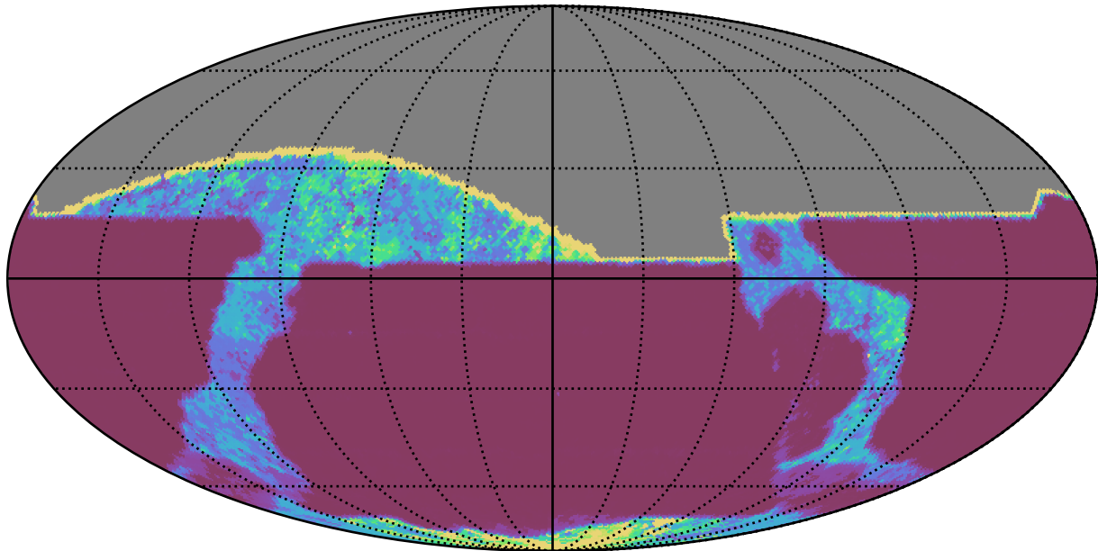
too_5_4v3.4_10yrs All sky all bands: 20thPercentile Inter-Night Gap
