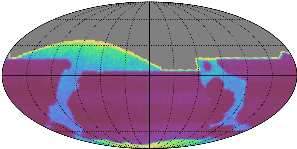
too_5_4v3.4_10yrs : properMotion
