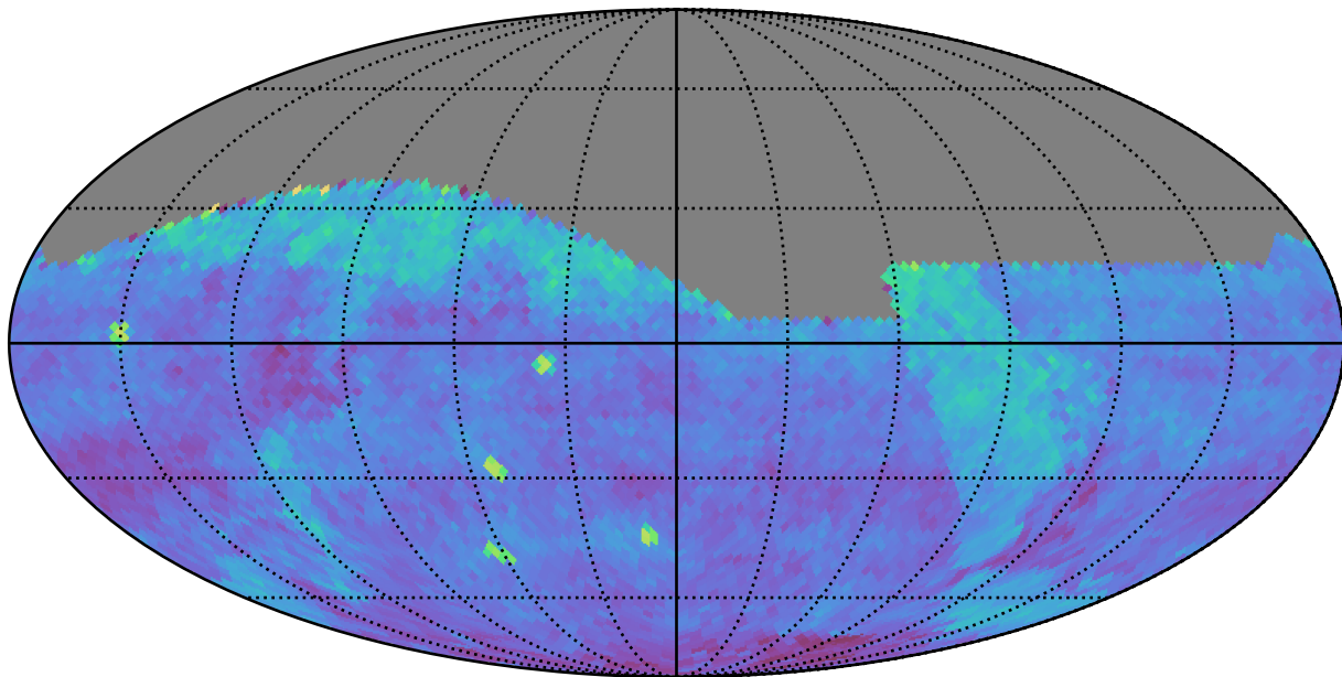
too_5_4v3.4_10yrs (g or r or i): PairFraction
