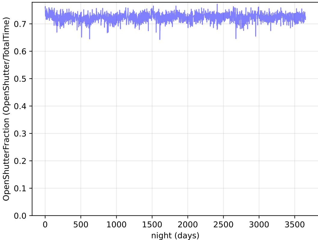
too_5_4v3.4_10yrs : OpenShutterFraction
