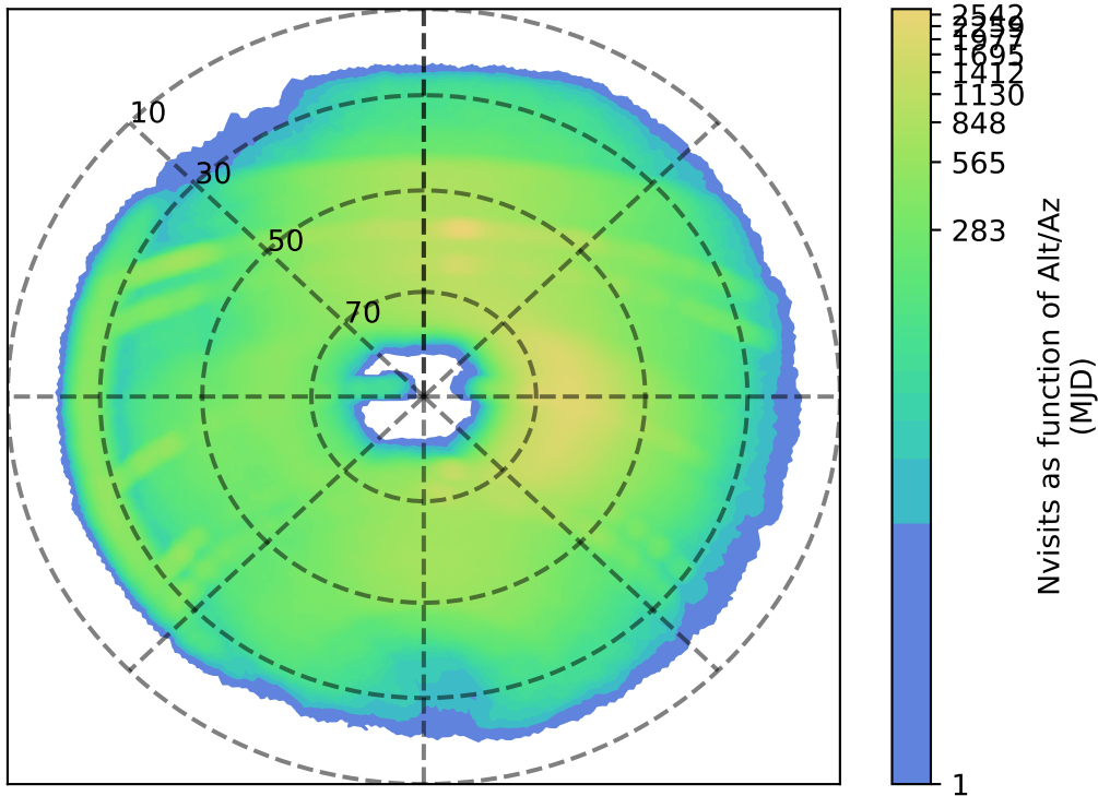
too_5_4v3.4_10yrs r: Nvisits as function of Alt/Az
