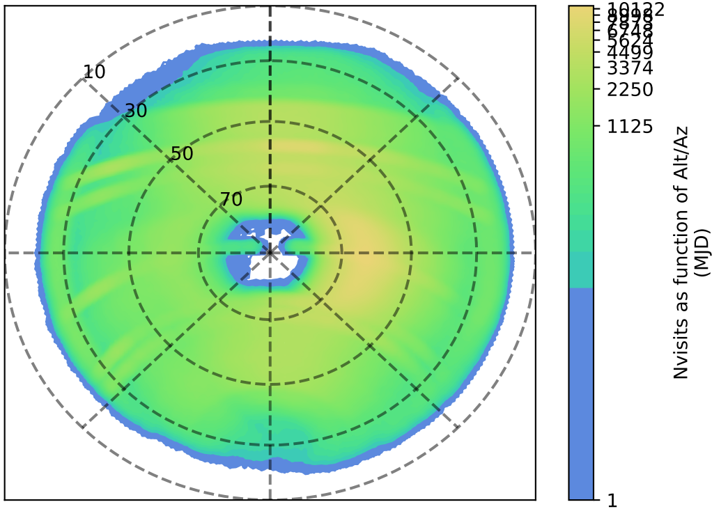
too_5_4v3.4_10yrs : Nvisits as function of Alt/Az
