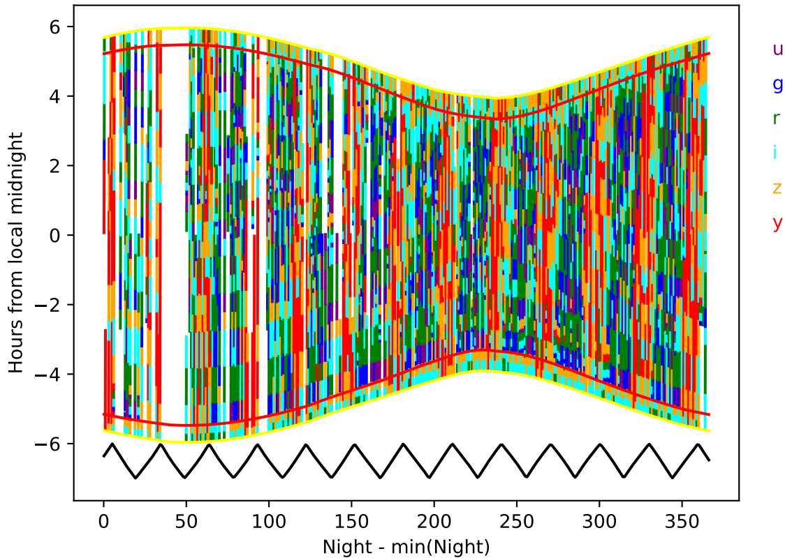
too_5_4v3.4_10yrs year 6-7: Hourglass
