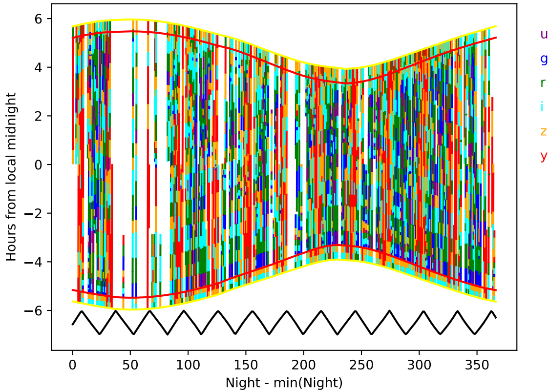
too_5_4v3.4_10yrs year 3-4: Hourglass
