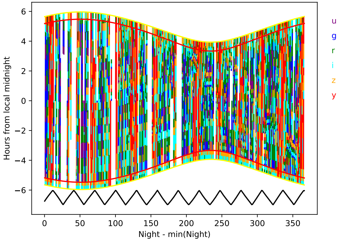
too_5_4v3.4_10yrs year 0-1: Hourglass
