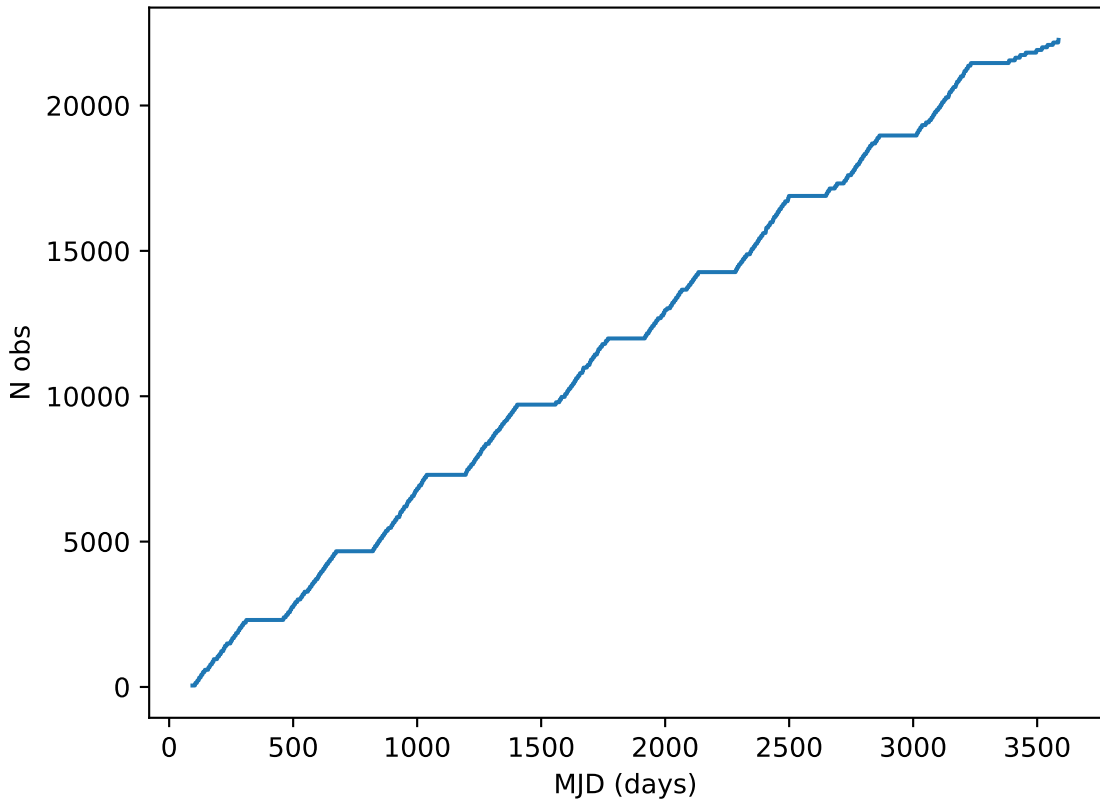
too_5_4v3.4_10yrs note like DD:ECDFS%: Cumulative
