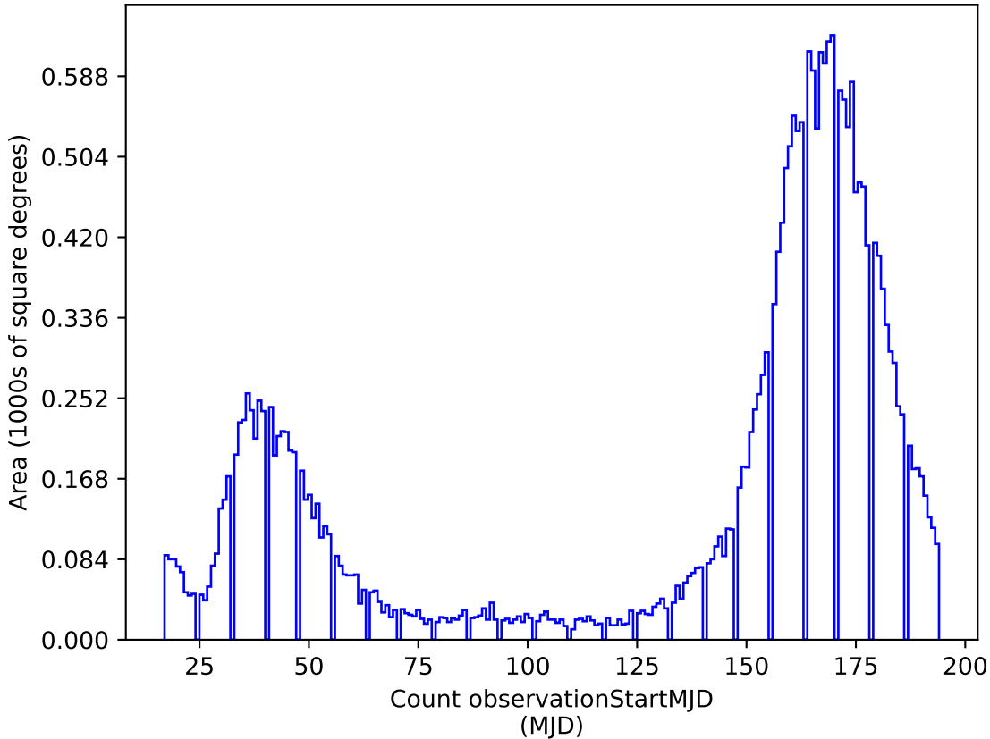
too_5_4v3.4_10yrs z: Count observationStartMJD
