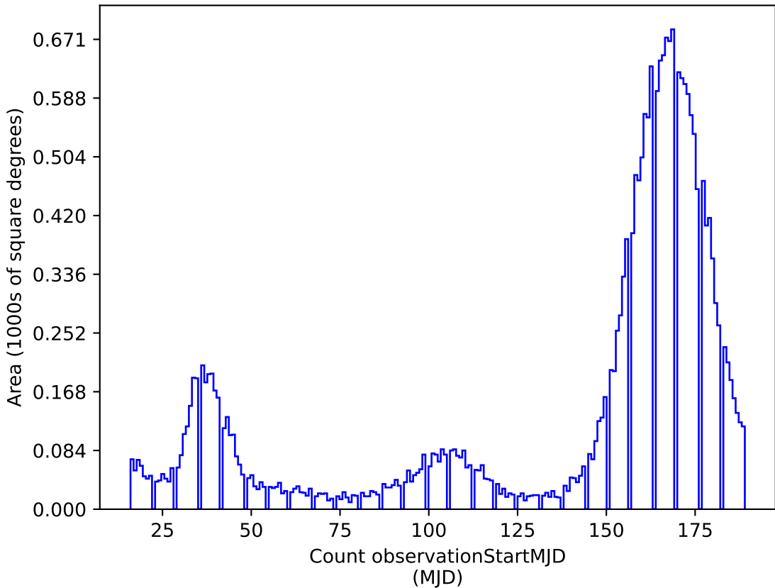
too_5_4v3.4_10yrs y: Count observationStartMJD
